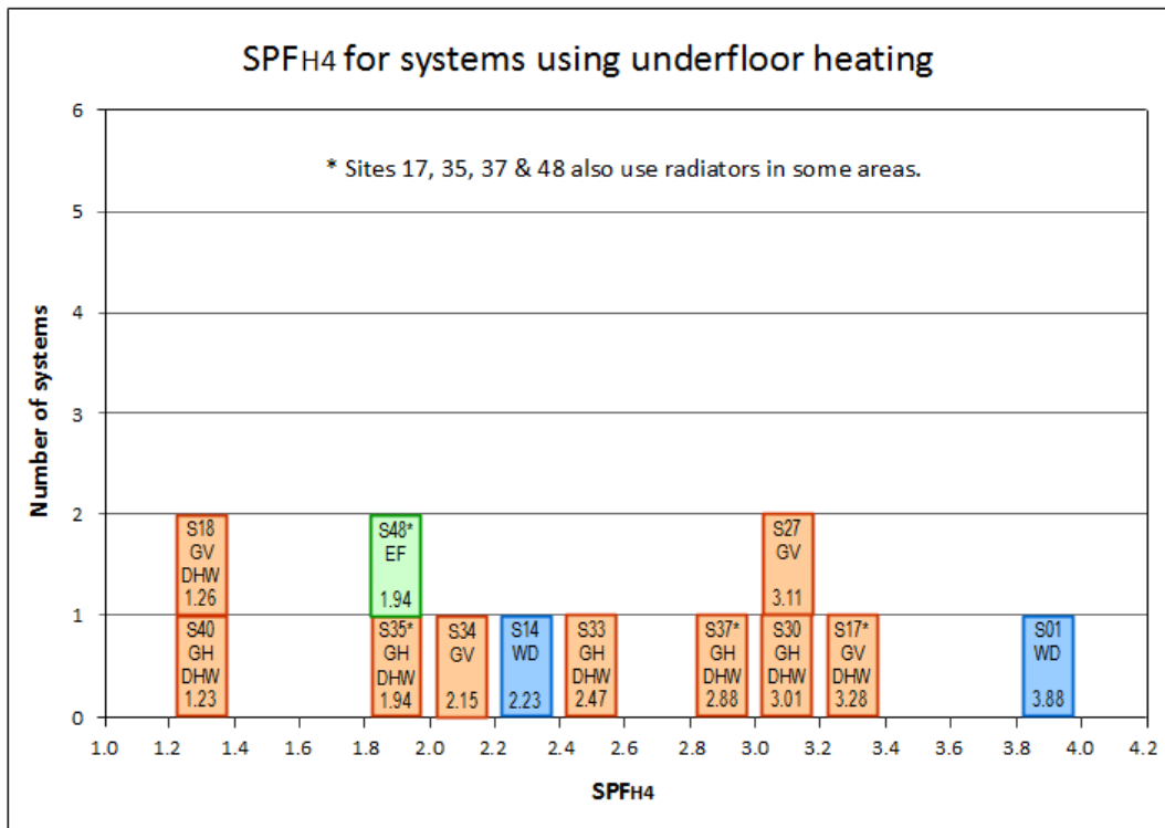
Figure 9 – Histogram of systems that use underfloor heating
