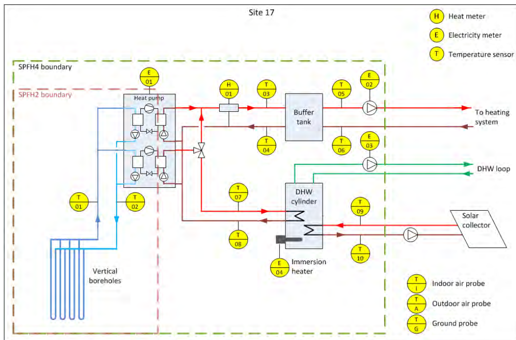
Figure 41 – Site 17 system schematic
